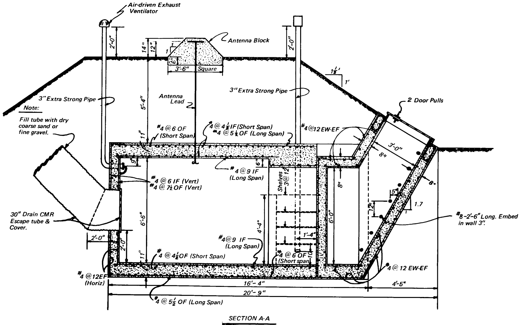
Fig. 2—Longitudinal section of FCDA family shelter, Mark I.
